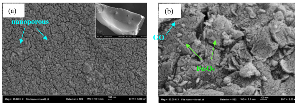
Figure 2: FESEM micrograph of (a) GO and (b) as-synthesised \text{GO-Fe}_3\text{O}_4
